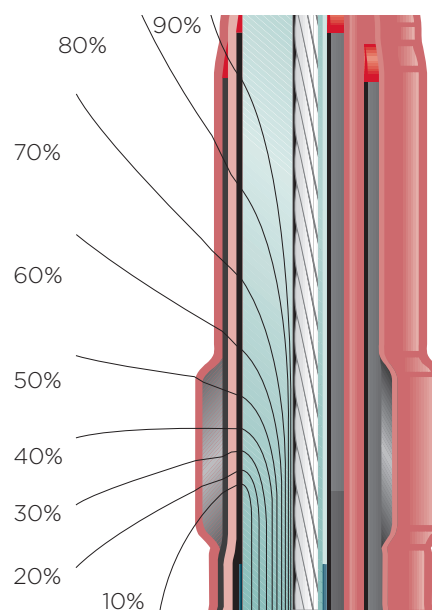
Stress control diagram
